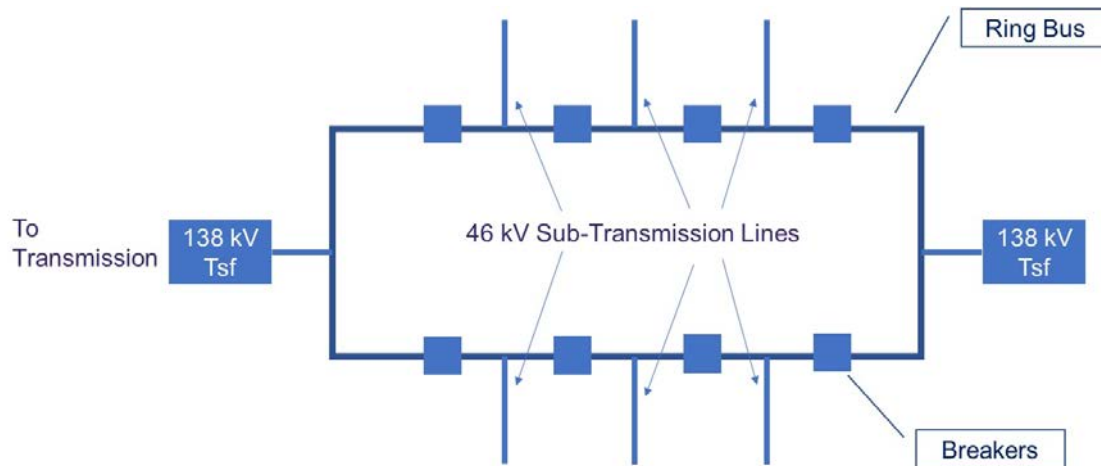
Figure J- 8: Waiau 46 kV GIS Bus
