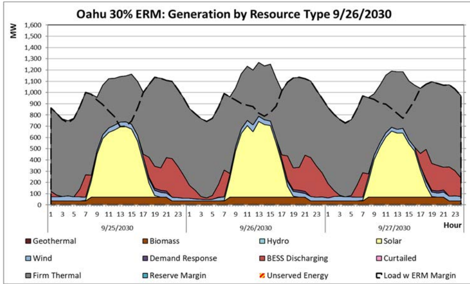
Figure C- 7: O’ahu Stochastic Outage Production Simulation Daily Chart
