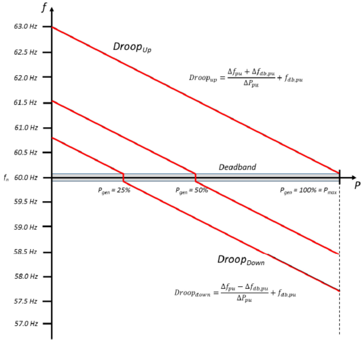
Figure B-2, Dynamic PFR Characteristic
