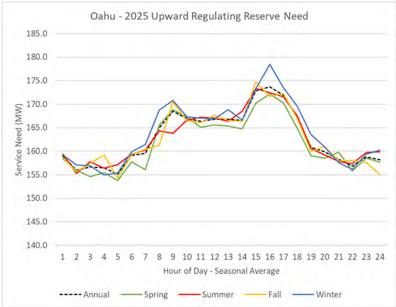
Figure 2: O’ahu 2025 Need for Upward Regulating Reserve
