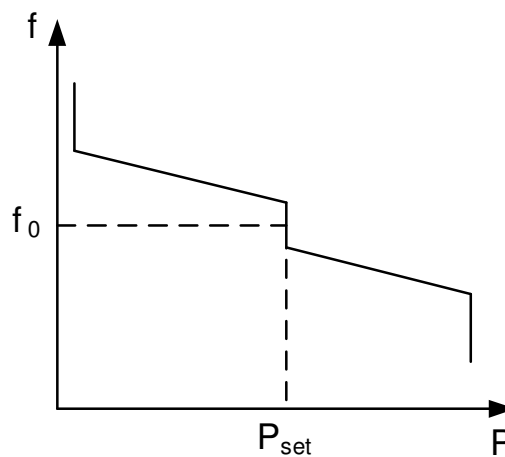
Figure 1 – Frequency Droop Control Characteristic with Deadband
