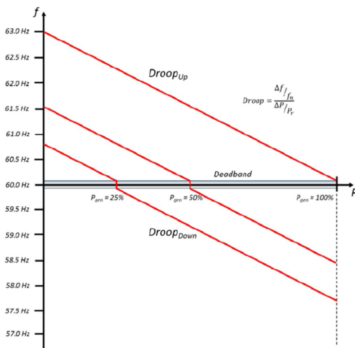
Active Power - Frequency Control Characteristic
